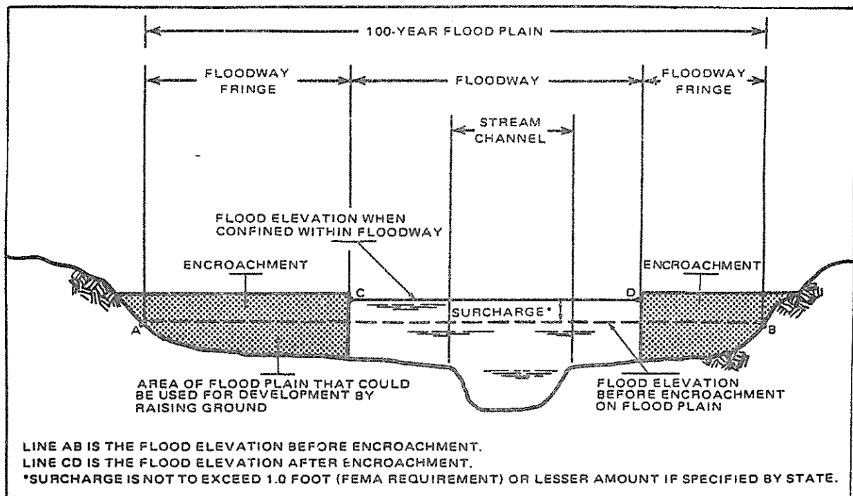
Figure 2. Floodway Schematic
